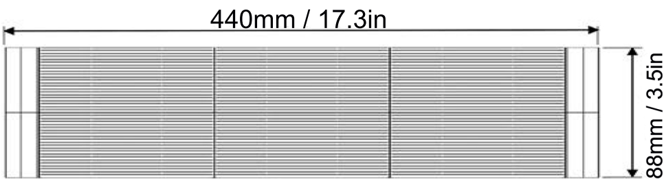
Front View
