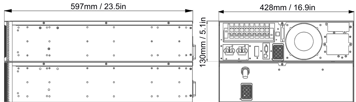
SIDE VIEW
